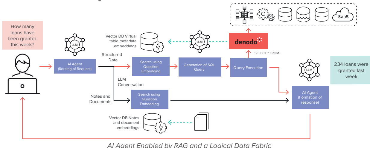
AI Agent Enabled by RAG and a Logical Data Fabric
